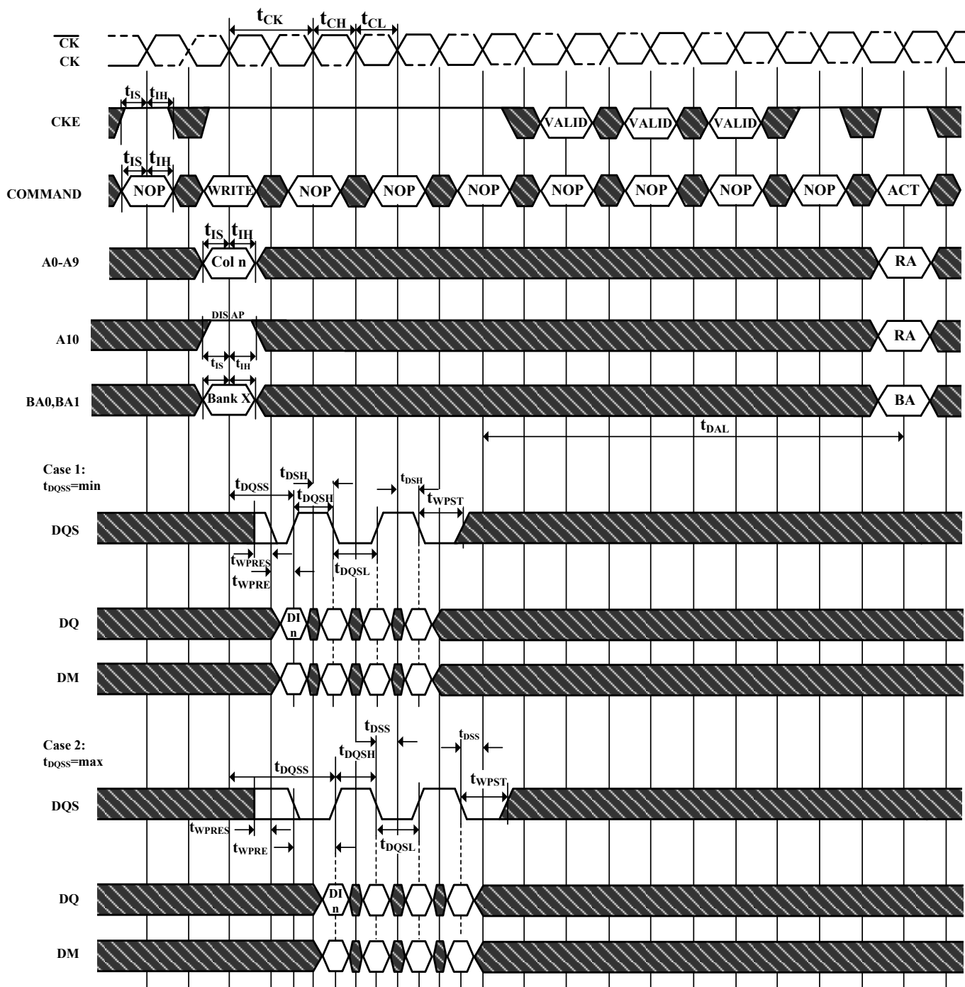
Figure 40. Write with Auto Precharge
